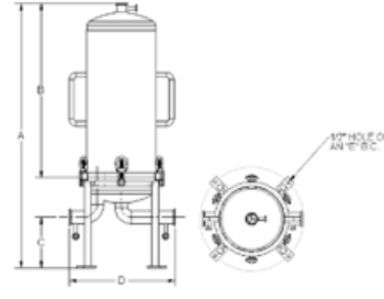
SRA T-Style Swing Bolt
